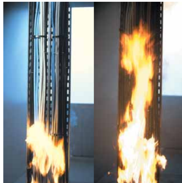
Test on conventional cables
